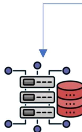
BD Manager
